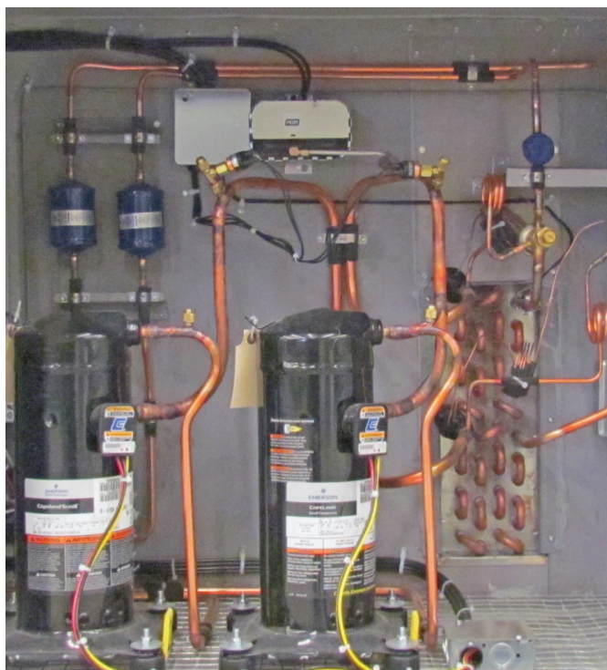
Compressor Section
