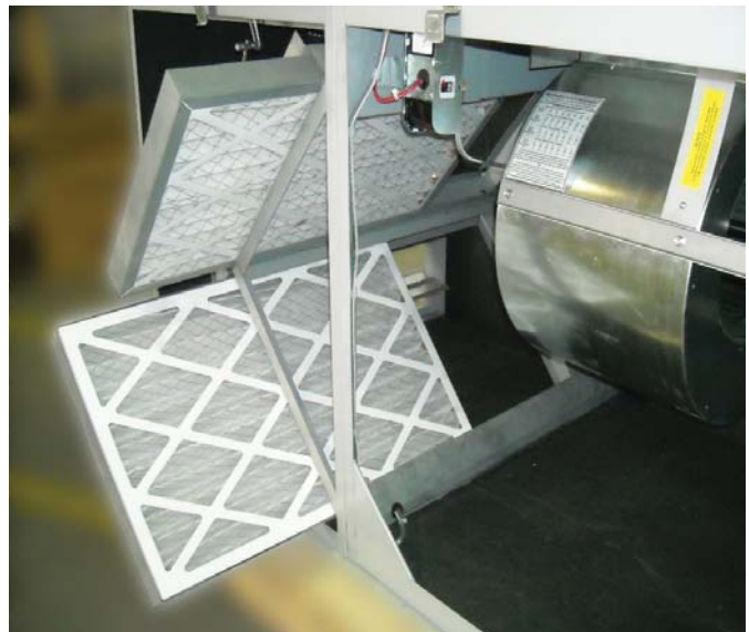
Slide out 2" (51 mm) pleated filters with metal frame
