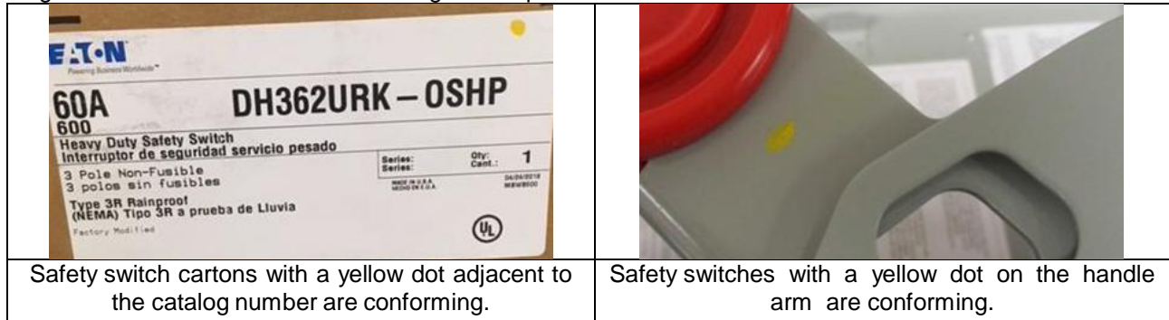
Figure 2. Identification of conforming switches (safety switches only). If any of the yellow markings as indicated below are present on your product, no return or repair is required. Switches containing this yellow marking have been verified to be conforming and require no further action.
