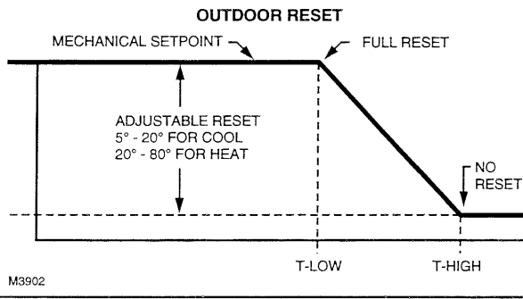
Fig. 19—Outdoor reset.
