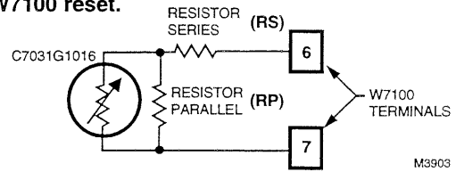
Fig. 20—Series/parallel resistance wiring for W7100 reset.
