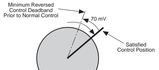
NF Actuator responds to a 70 mV signal when reversing direction from stop position.
